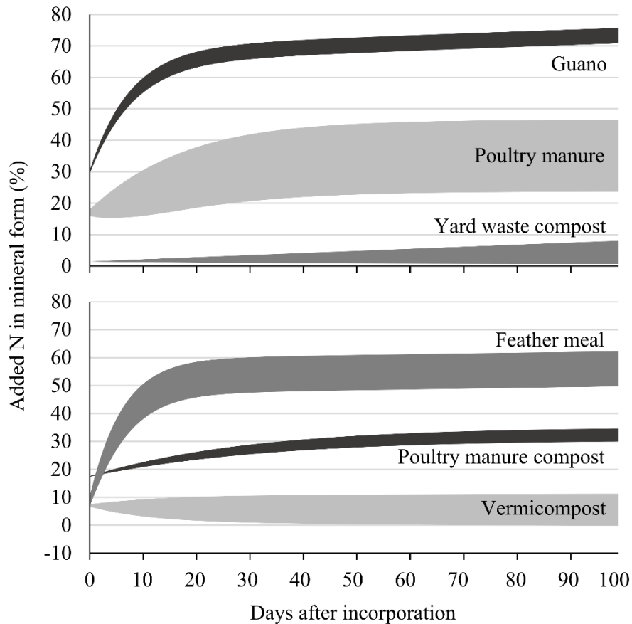
Figure 2. Simulated N turnover from organic fertilizers and composts based on minimum and maximum C:N ratios from a literature survey. The calculations assumed optimal moisture content and a constant temperature of 77 °F (Geisseler et al., 2021).
